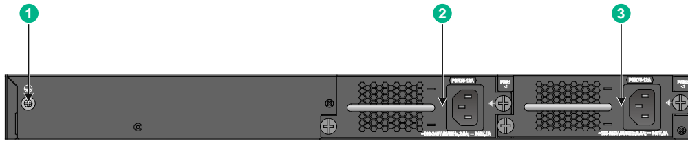
Figure2-2 Rear panel
