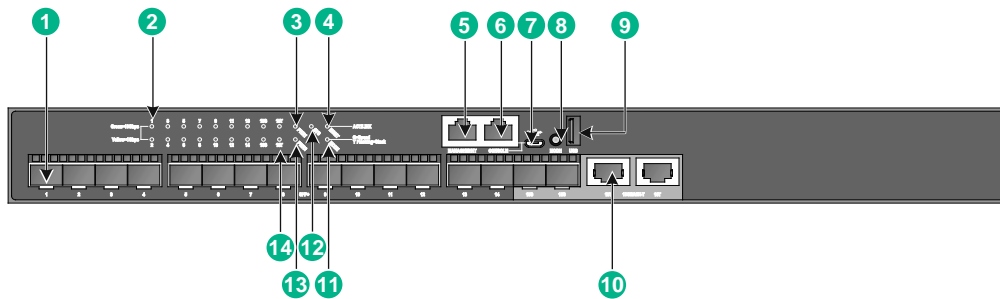
Figure2-1 Front panel
