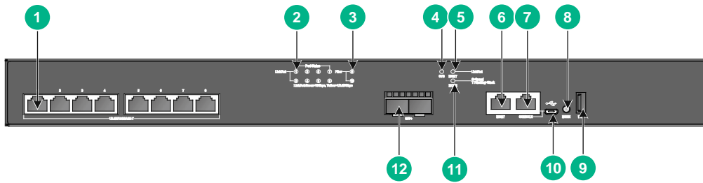
Figure2-5 Front panel
