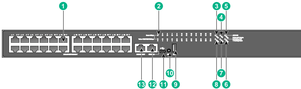
Figure2-15 Front panel
