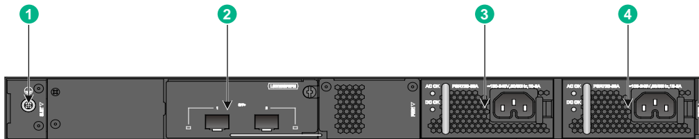
Figure2-16 Rear panel
