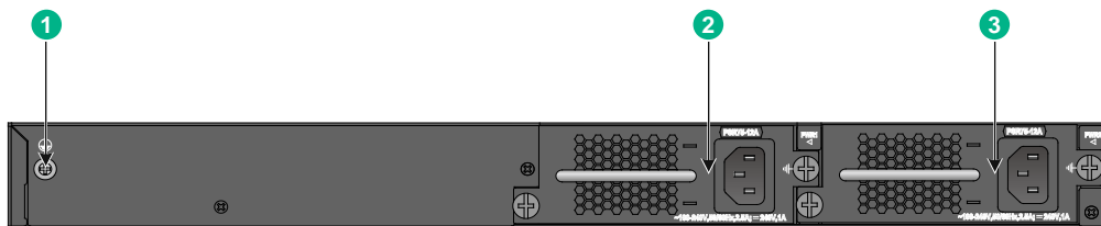
Figure2-4 Rear panel
