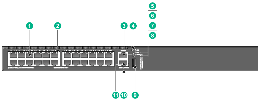
Figure2-17 Front panel
