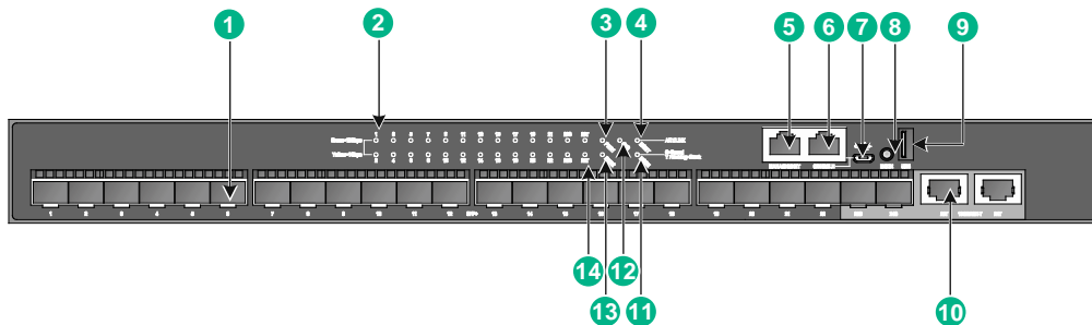
Figure2-3 Front panel
