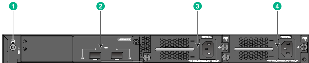
Figure2-14 Rear panel
